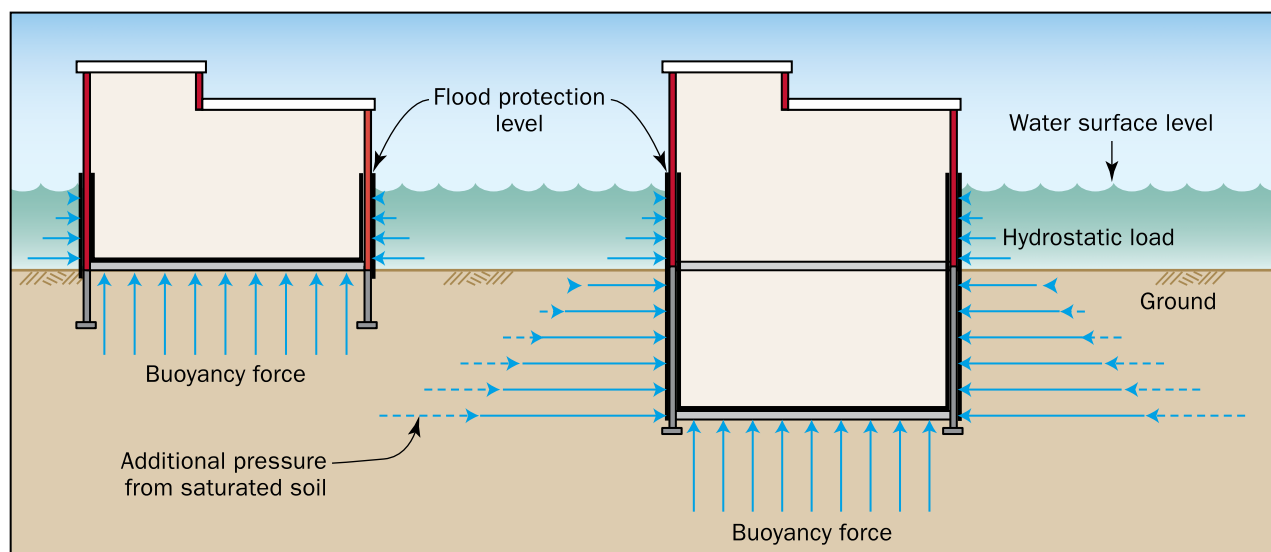
Figure 3: Hydrostatic loads
