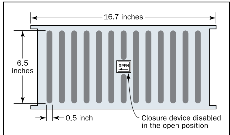
Figure 18: Example of non-engineered opening: Typical standard air vent faceplate providing 42 square inches of net open area if disabled in the open position; measurement of net open area uses a slot width of 0.5 inch times a slot height of 6.5 inches times the total number of slots
